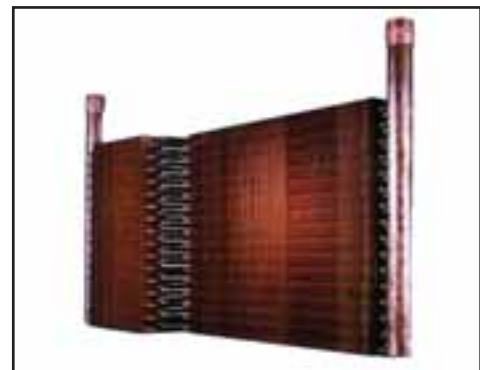
Dryer Coils with offset connections. Replacement design for bent tubes.
